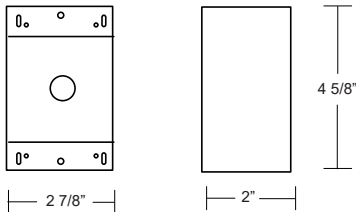
Back Box (OPTIONAL)
